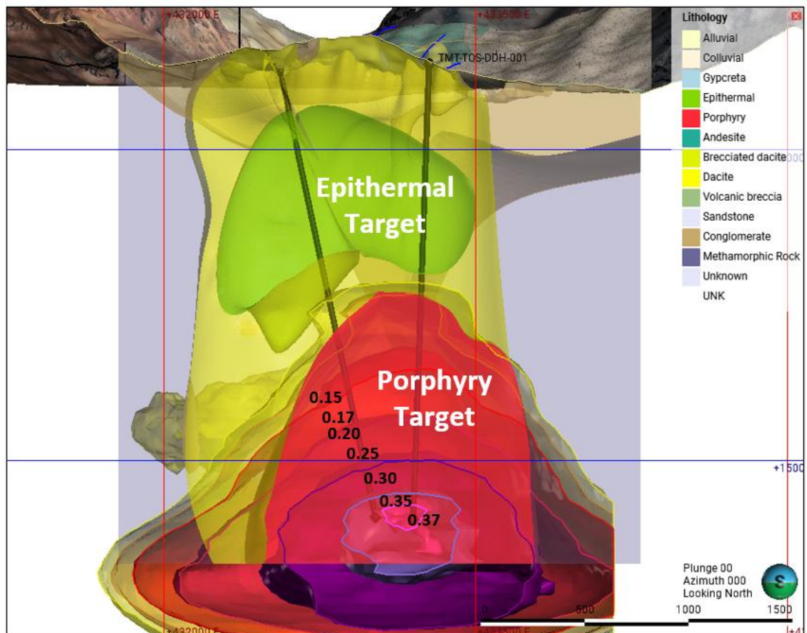
Figure 4: Geological cross section (looking north) for the Toro South target (see figure 3 for plan view location), showing indicative drill holes TMT-TOS-DDH-001 and TMT-TOS-DDH-002 targeting interpreted epithermal and porphyry targets. Note: The numbers on the iso surfaces represent probability scores (0-1) of the geochemical models at Tambo matching with the reference metal-zoning models from Cohen (2011). Values over 0.15 are considered 'significant', with a maximum score of 1.00, which corresponds to a 100% match.
