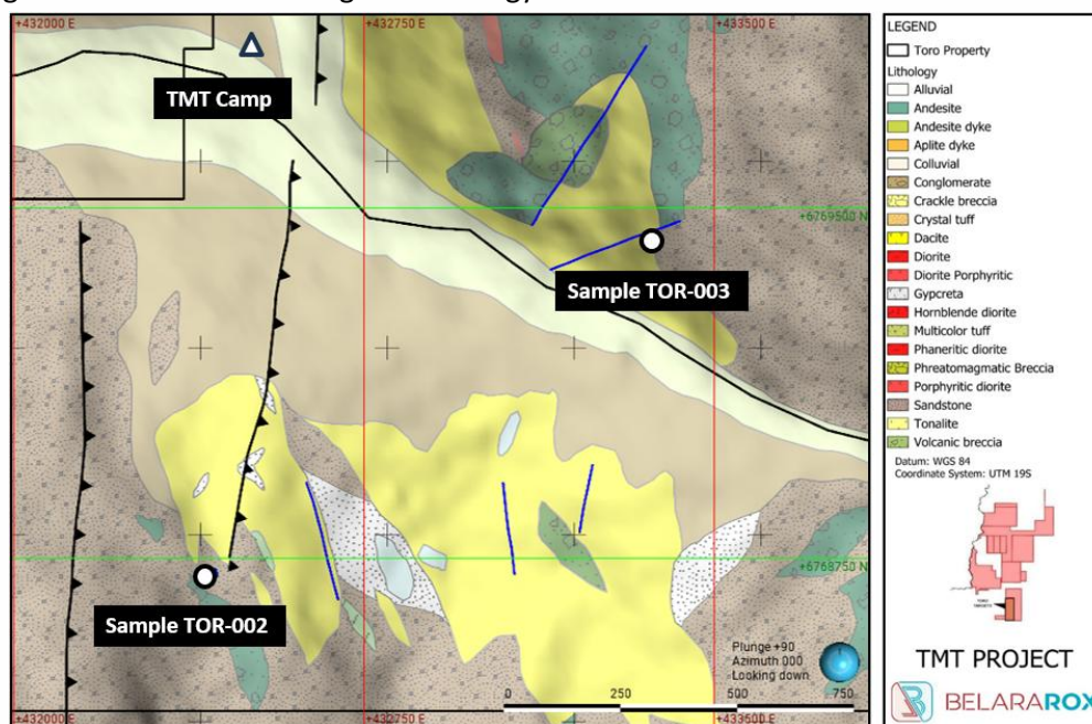
Figure 7: Location of samples TOR-002 and TOR-003 at the Toro prospect.
