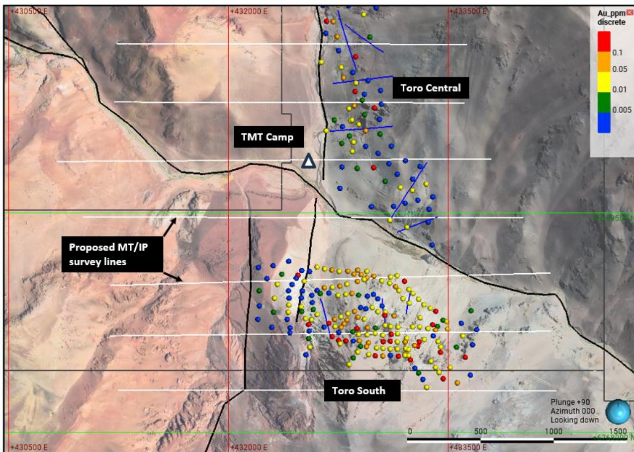
Figure 5: Proposed survey lines (white lines) for the MT/IP geophysical survey over an area of approximately 2500m by 2500m covering the entire Toro South target and the most prospective zones of the Toro Central target.
