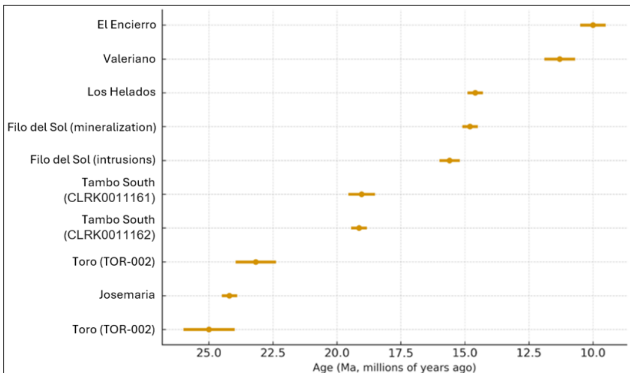
Figure 9: Interpreted magmatic ages from Toro and Tambo South compared with major Cu deposits nearby. Baseline deposit ages derived from Perello et al. (2023).
