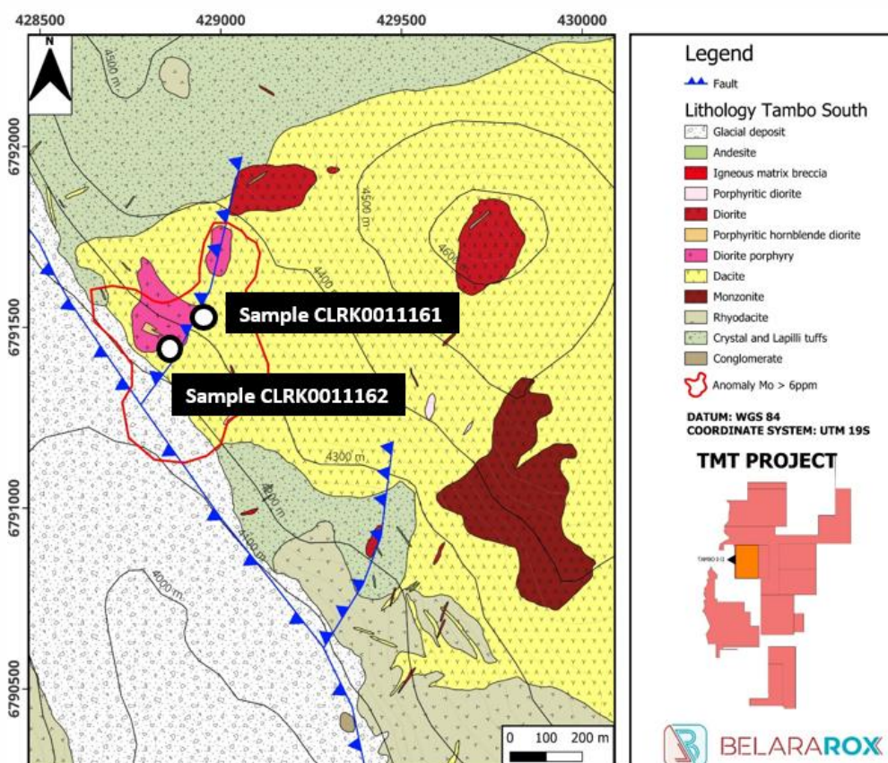
Figure 8: Location of samples CLRK0011161 and CLRK0011162 at the Tambo South prospect.
