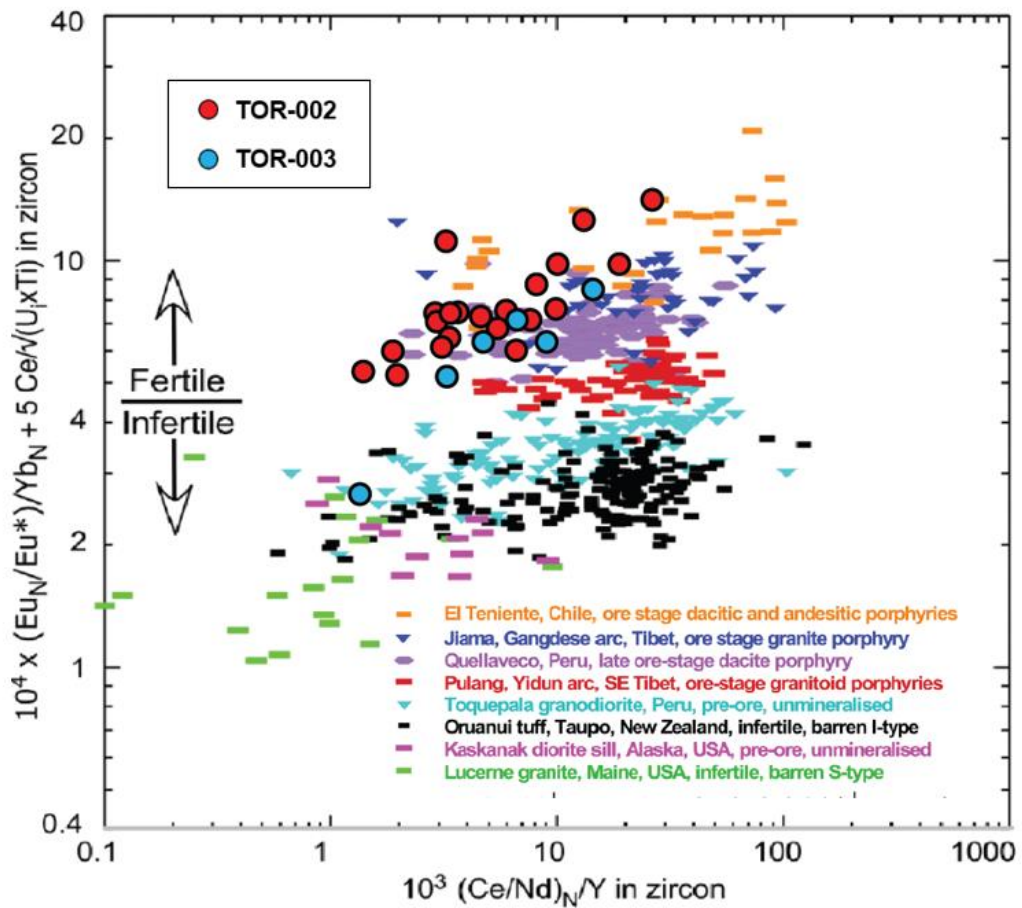
Figure 10: Zircons from samples TOR-002 and TOR-003 are plotted against zircons from ore-stage intrusions in four porphyry copper deposits (El Teniente, Jiama, Quellaveco, and Pulang) are compared with zircons in pre-ore intrusions (Toquepala Granodiorite in Peru and Kaskanak diorite in the Pebble district, Alaska), and in infertile igneous units in unmineralized regions (Oruanui rhyolite tuff, Lucerne granite). After Loucks et al. (2024).
